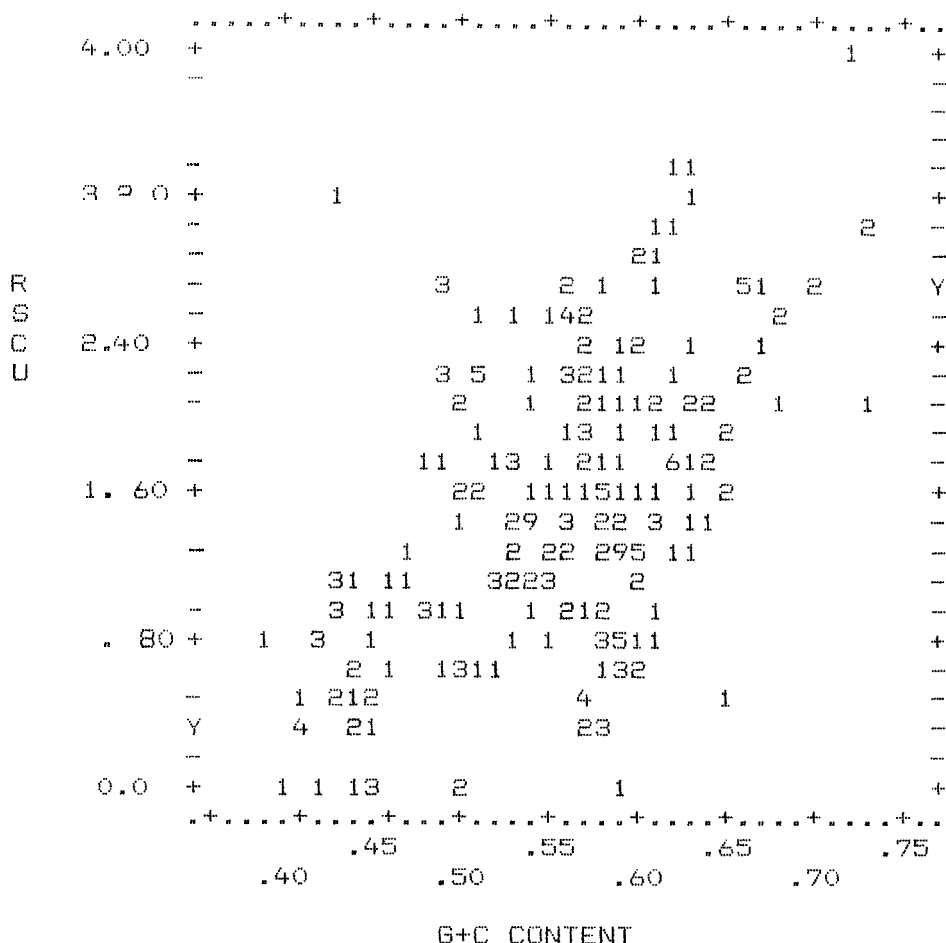
Fig. 1 RSCU values of the CGC codon(Arg4) plotted against the G+C content (G+C/G+C+A+U) of the coding sequence in human genes. The regression line may be drawn connecting the Y marks on the plot frame. No. of genes = 277, correlation coefficient = .511, slope = 5.76.
